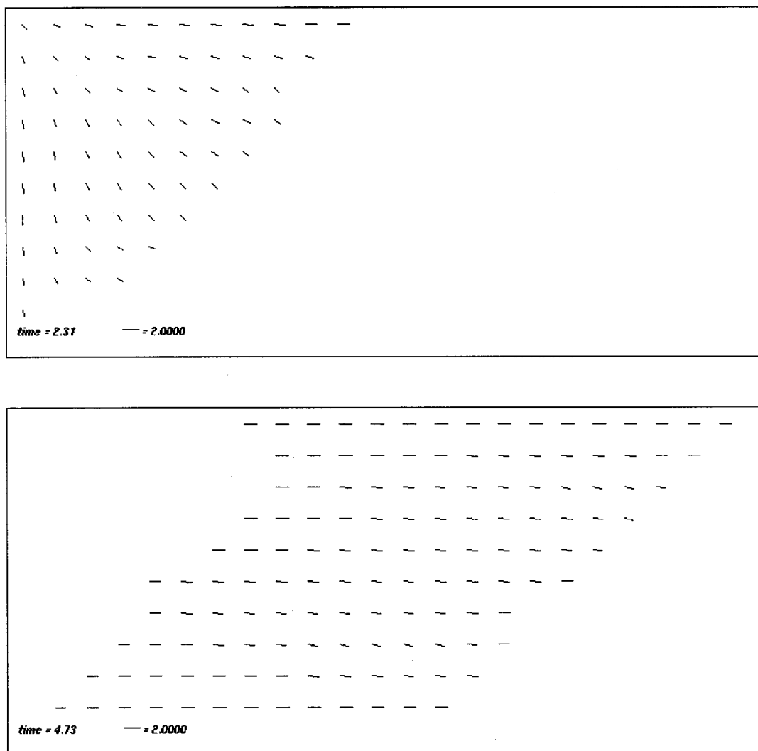
Fig. 11. Time slices from the movement of a line behind a rectangular aperture illustrating the two phases of motion in the barberpole illusion. Each graphic shows long-range filter cell activity interpreted as motion vectors. In the first time slice, the line moves through the corner region, and signals in the line interior indicate motion perpendicular to the line's orientation. Feature signals dominate the output near the aperture edges but do not dominate the ambiguous motion signals along the rest of the line. In the later time slice, motion is captured by feature motion signals in the direction coincident with the long axis of the aperture.
