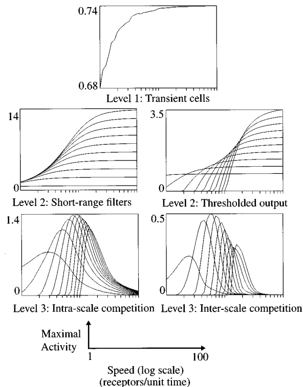
Fig. 5. Maximal response of one-dimensional model cells to a range of simulated speeds. For levels where there are multiple spatial scales at each position, activities from different scales are shown as different curves superimposed on the same plot. The smaller scales tend to respond less vigorously to fast speeds. See the text for details.
