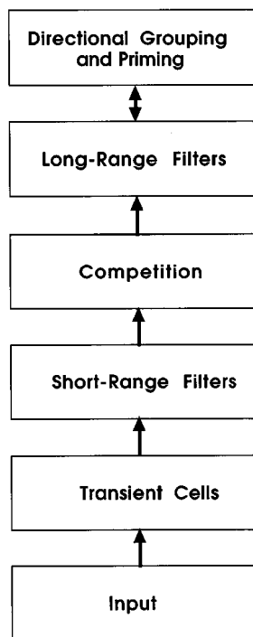
Fig. 4. Model processing stages. See the text for details.
