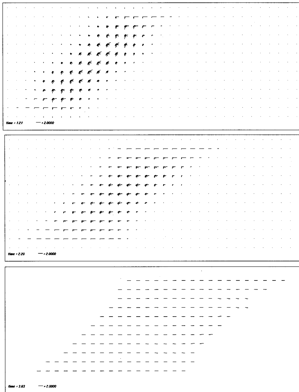
Fig. 9. Maximal activities across all scales of the long-range filters during the rightward motion of a 45-deg line at three successive times. Ambiguous motion signals are eliminated by feedback inhibition from the long-range directional grouping cells.
