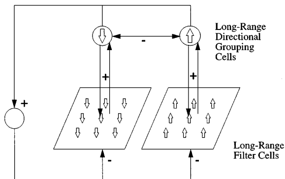
Fig. 8. Long-range directional grouping and feedback in which each grouping cell nonspecifically inhibits all long-range filters while exciting cells with the same directional preference.
