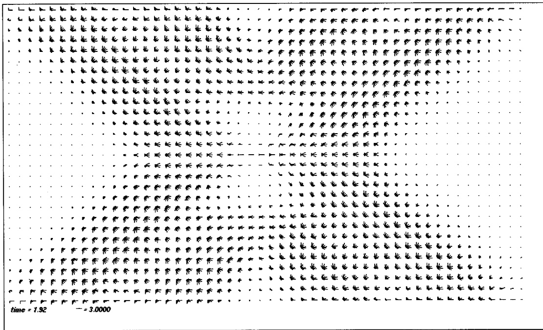
Fig. 14. Long-range filter responses combining On and Off channels during simulated motion of a type 1 symmetric plaid. Components are aligned at 45 deg from vertical. Filter responses have been magnified to show ambiguous signals clearly. The large feature signals do not therefore appear at their true magnitude. Such feature signals are present at the four corners, where the components intersect.
