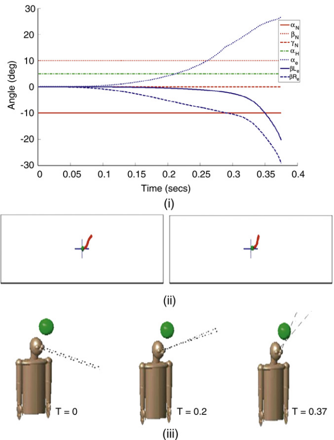
Fig. 8. This shows an example saccade sequence with loss of the entire head and neck movement. (i) Joint position trajectories during the saccade. (ii) Spatial trajectory of the target in the stereo camera during the saccade. (iii) Initial, intermediate and final images of system during saccade.
