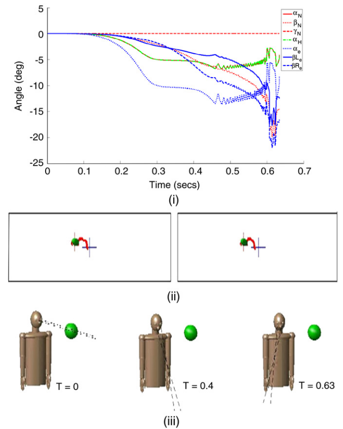
Fig. 7. This shows an example saccade sequence with loss of \gamma_N and a change in the image center (the red cross hair indicates the new center). (i) Joint position trajectories during the saccade. (ii) Spatial trajectory of the target in the camera during the saccade. (iii) Initial, intermediate and final images of system during saccade.
